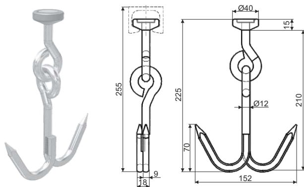
Hák dvojitý s kĺbom Articulated double meat hook
